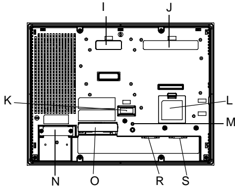
背面図 (AGP-3500L/3500S)
