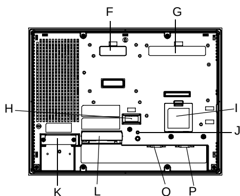
背面図 (AGP-3500L/3500S)
