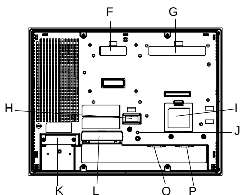
背面図 (AGP-3500L/3500S)
