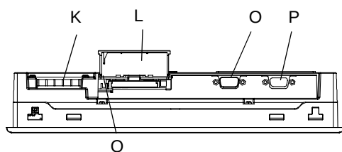
底面図 (AGP-3500L/3500S)
