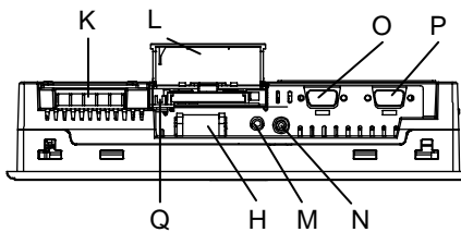
底面図 (AGP-3500T/3550T)
