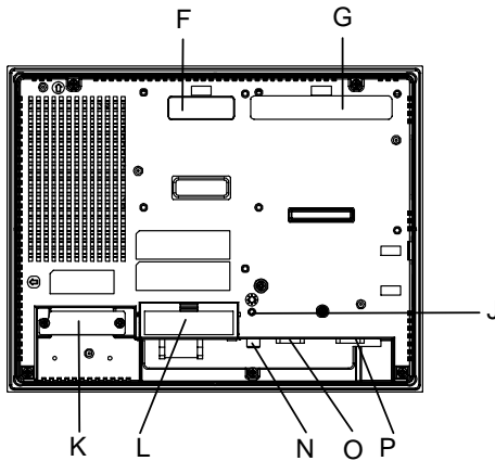
背面図 (AGP-3500T/3550T)
