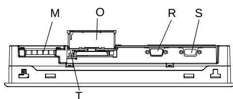
底面図 (AGP-3500L/3500S)
