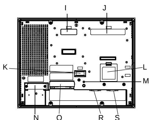
背面図 (AGP-3500L/3500S)
